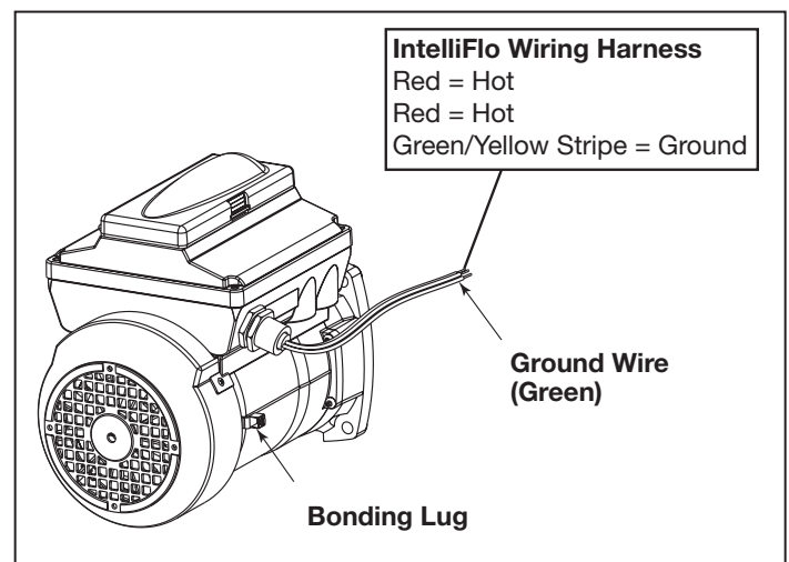
Figure 11. Pentair External Bonding
