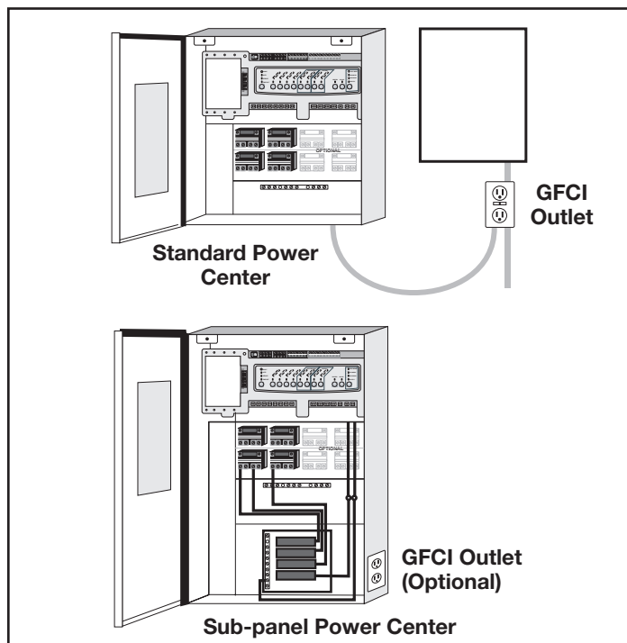
Figure 6. GFCI Installation for High Voltage Underwater Lighting
