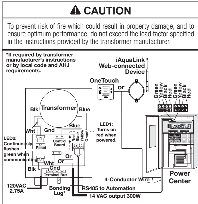
Figure 9. Wiring LED Lights to the Infinite WaterColors LED Light Controller
